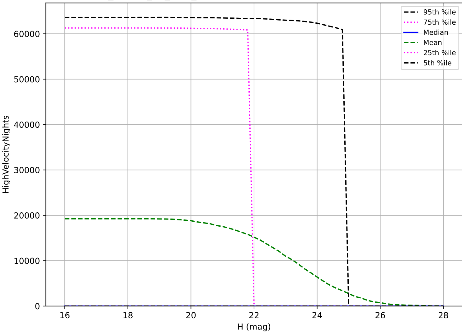
ddf_loaded_fl2_v3.4_10yrs: NEO High velocity pair detection loss
