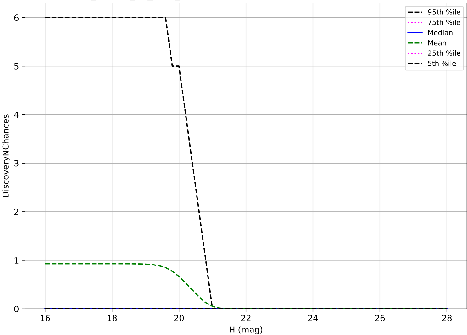
ddf_loaded_fl2_v3.4_10yrs: Vatira 3 pairs in 15 nights detection loss
