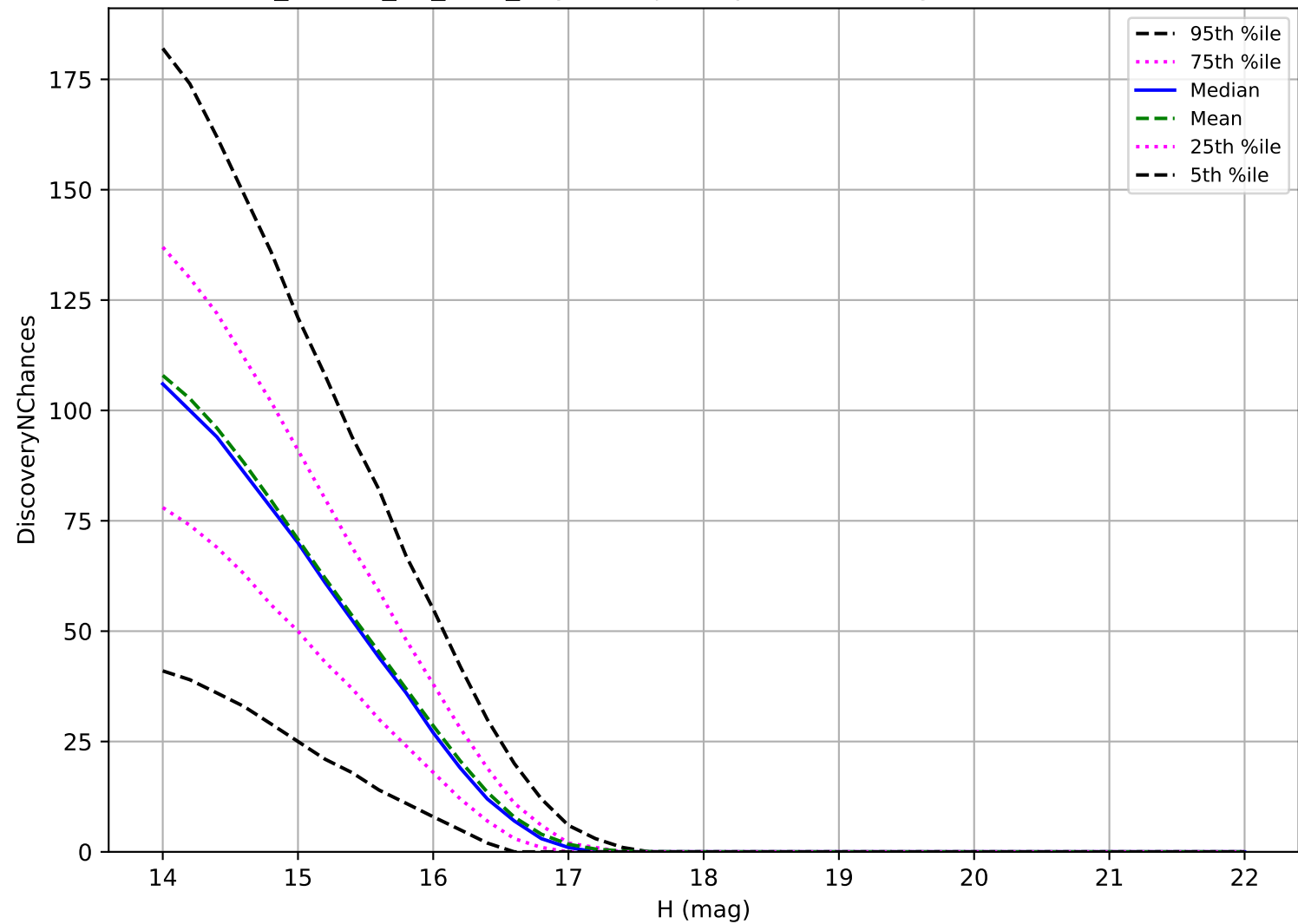
ddf_loaded_fl2_v3.4_10yrs: Trojan 3 pairs in 15 nights detection loss
