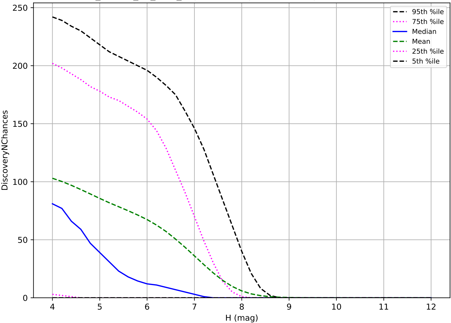
ddf_loaded_fl2_v3.4_10yrs: TNO 3 pairs in 15 nights detection loss
