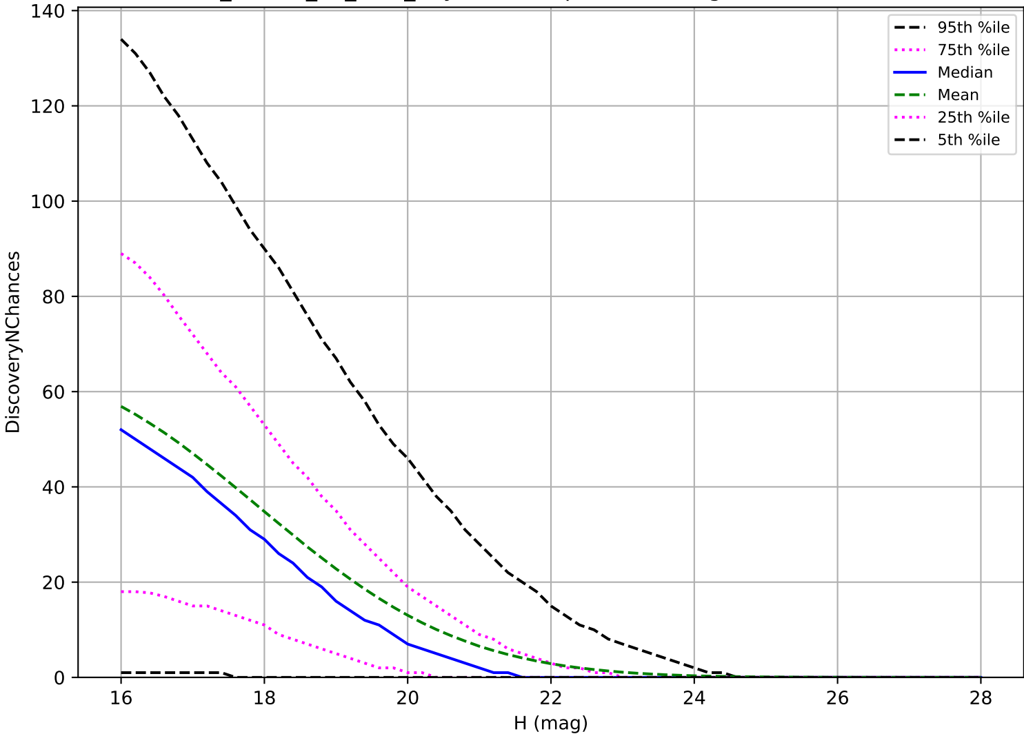
ddf_loaded_fl2_v3.4_10yrs: PHA 3 pairs in 15 nights detection loss
