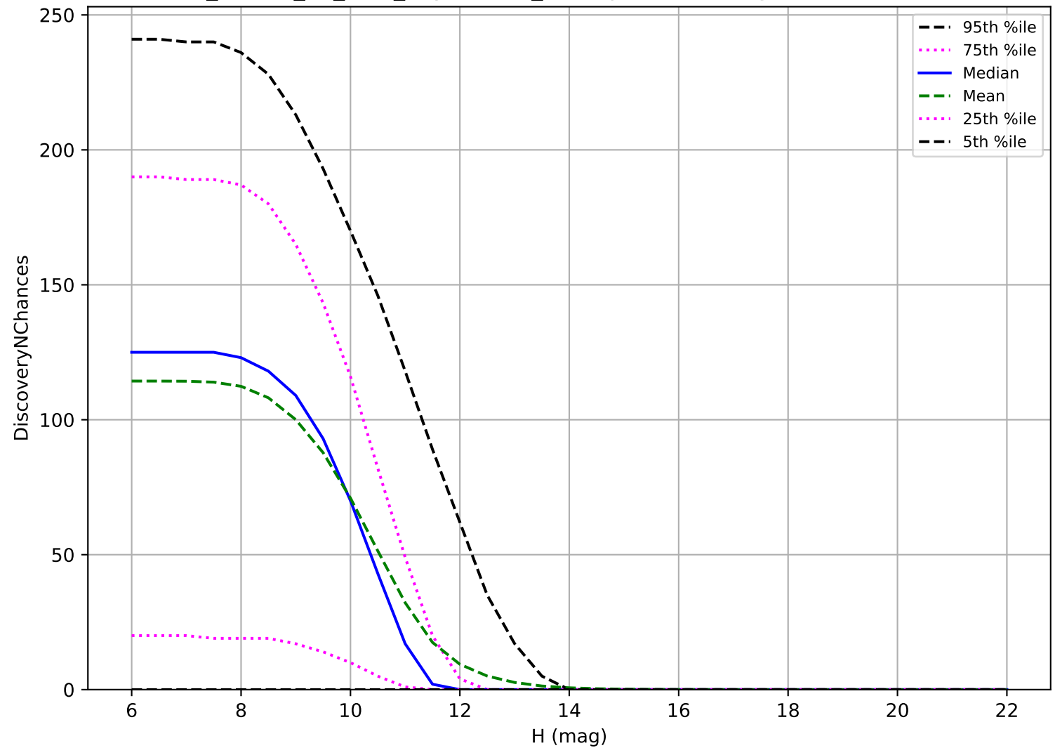
ddf_loaded_fl2_v3.4_10yrs: OCC_r20 3 pairs in 15 nights detection loss
