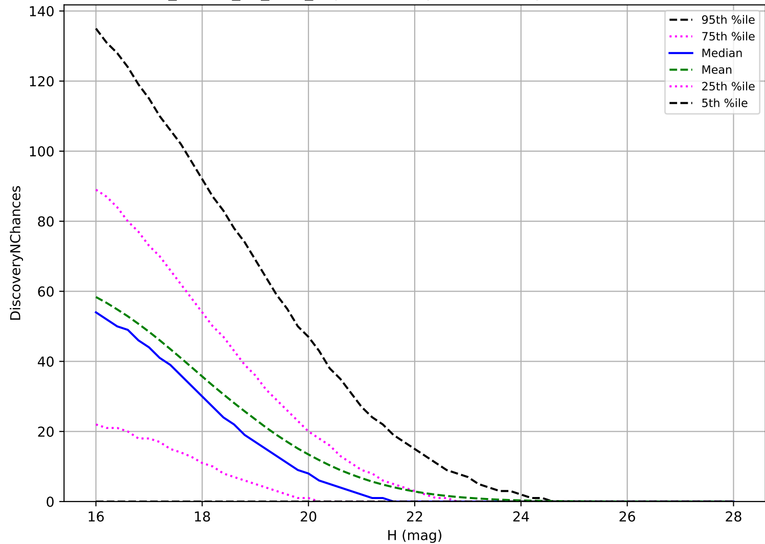
ddf_loaded_f12_v3.4_10yrs: NEO 3 pairs in 15 nights detection loss
