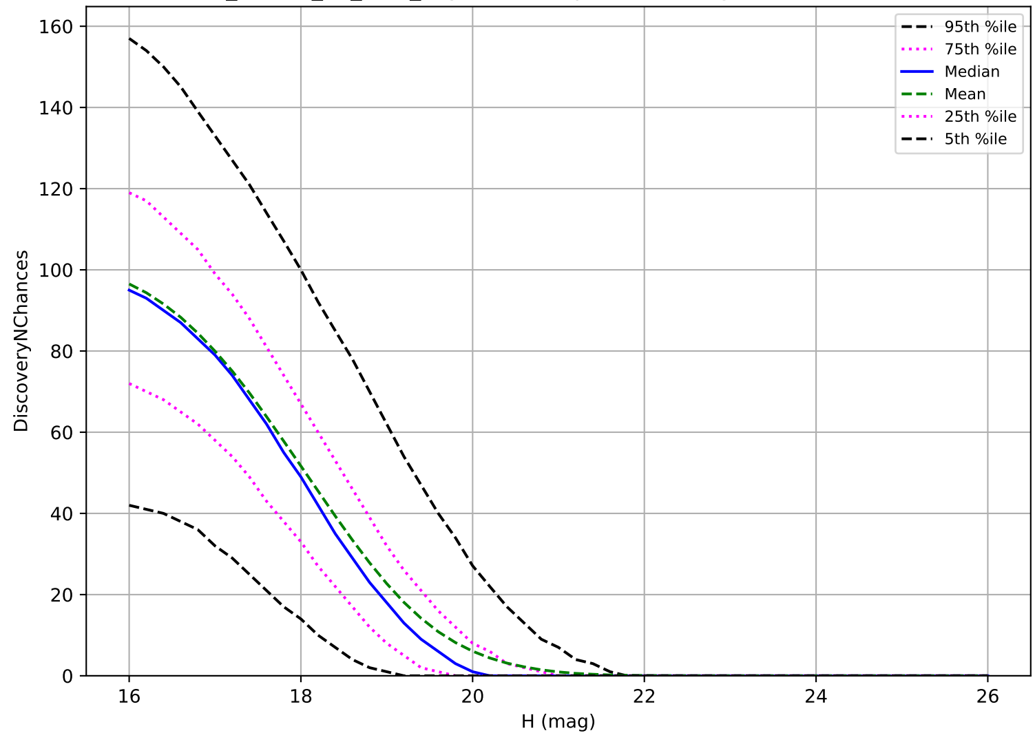
ddf_loaded_fl2_v3.4_10yrs: MBA 3 pairs in 15 nights detection loss
