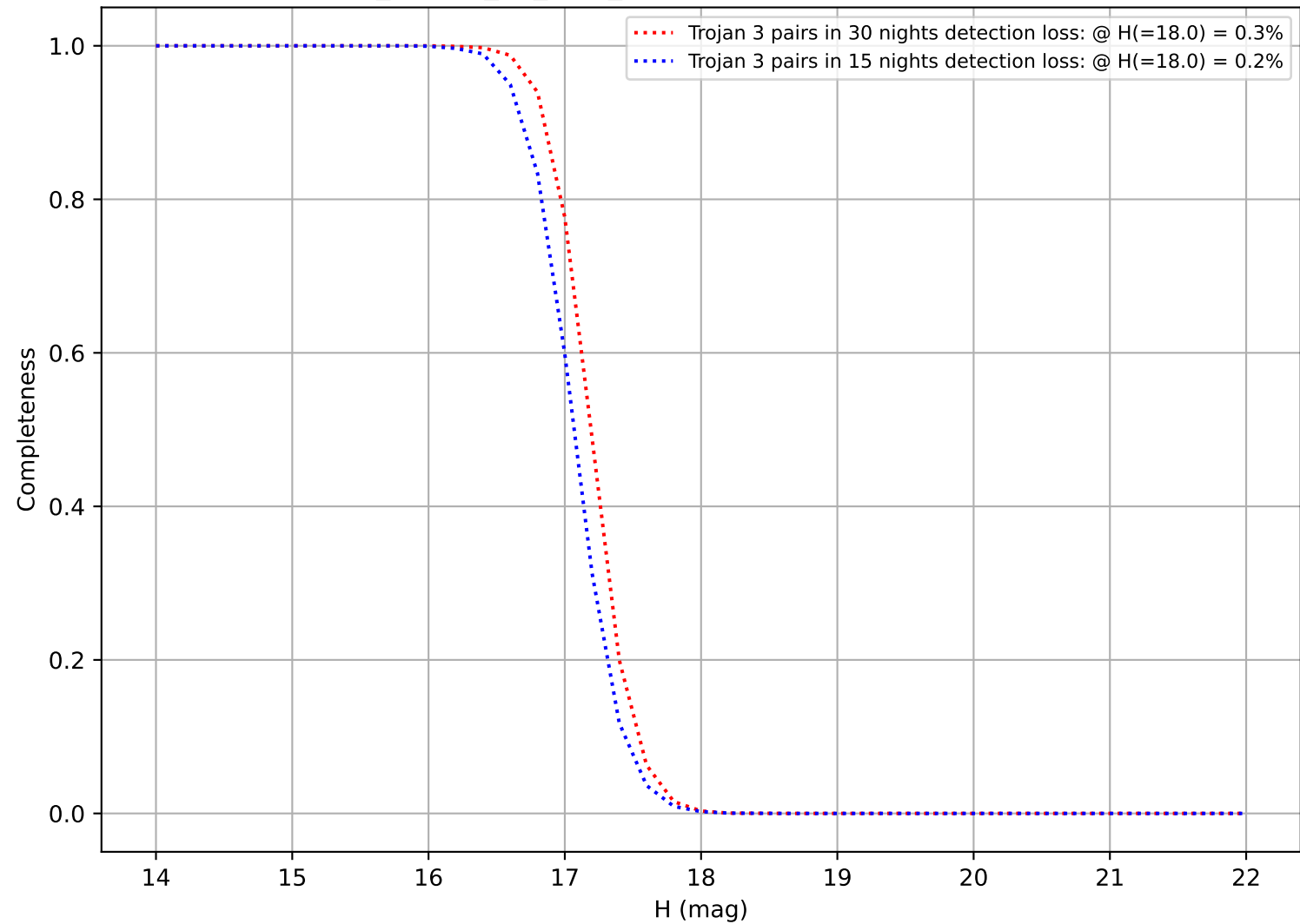
ddf_loaded_fl2_v3.4_10yrs: DifferentialCompleteness
