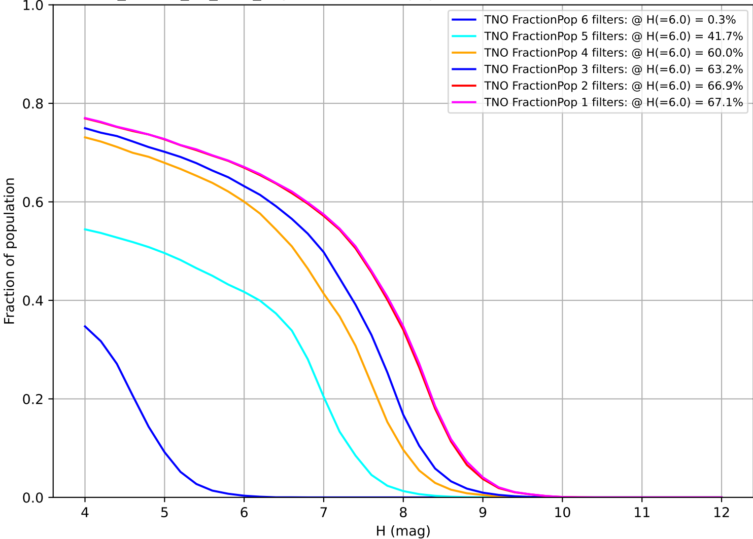
ddf_loaded_fl2_v3.4_10yrs: Fraction of population with colors in X filters TNO
