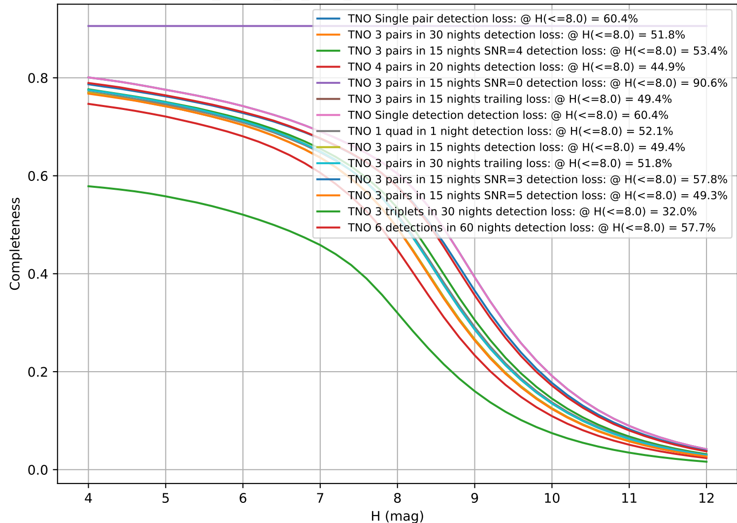
ddf_loaded_fl2_v3.4_10yrs: CumulativeCompleteness
