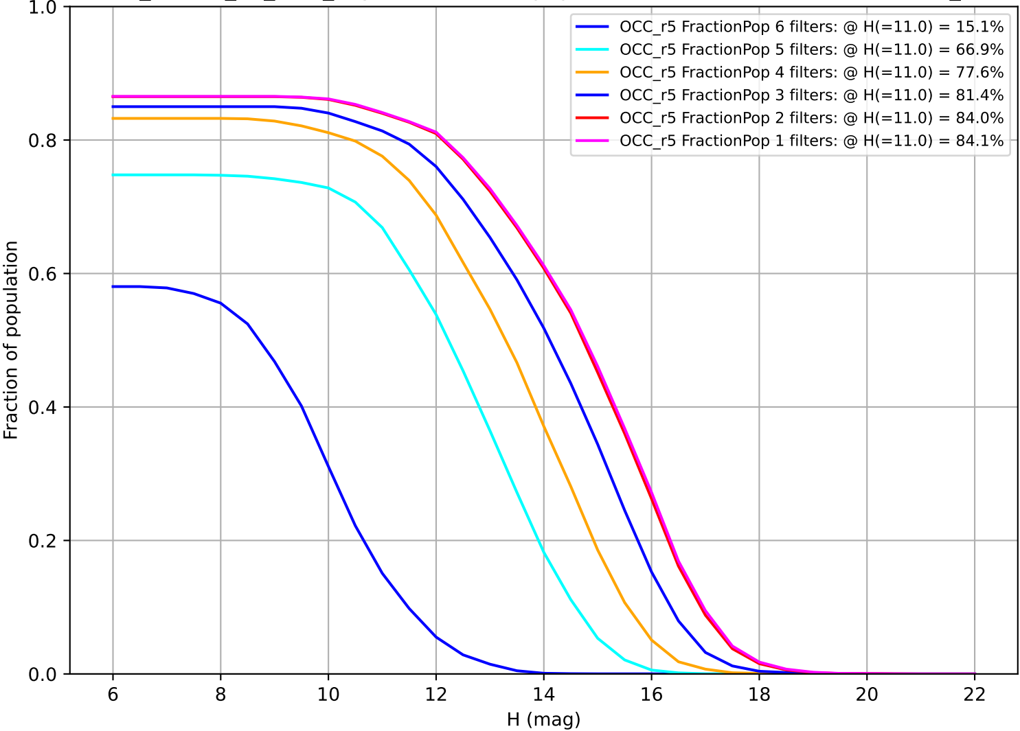
ddf_loaded_fl2_v3.4_10yrs: Fraction of population with colors in X filters OCC_r5
