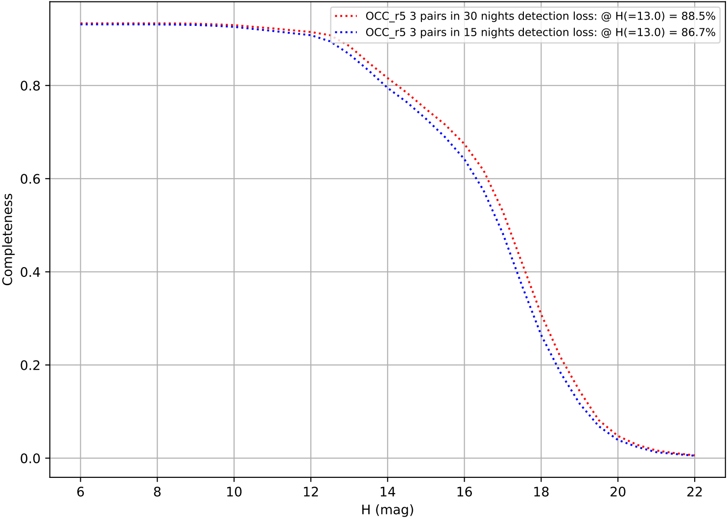
ddf_loaded_fl2_v3.4_10yrs: DifferentialCompleteness
