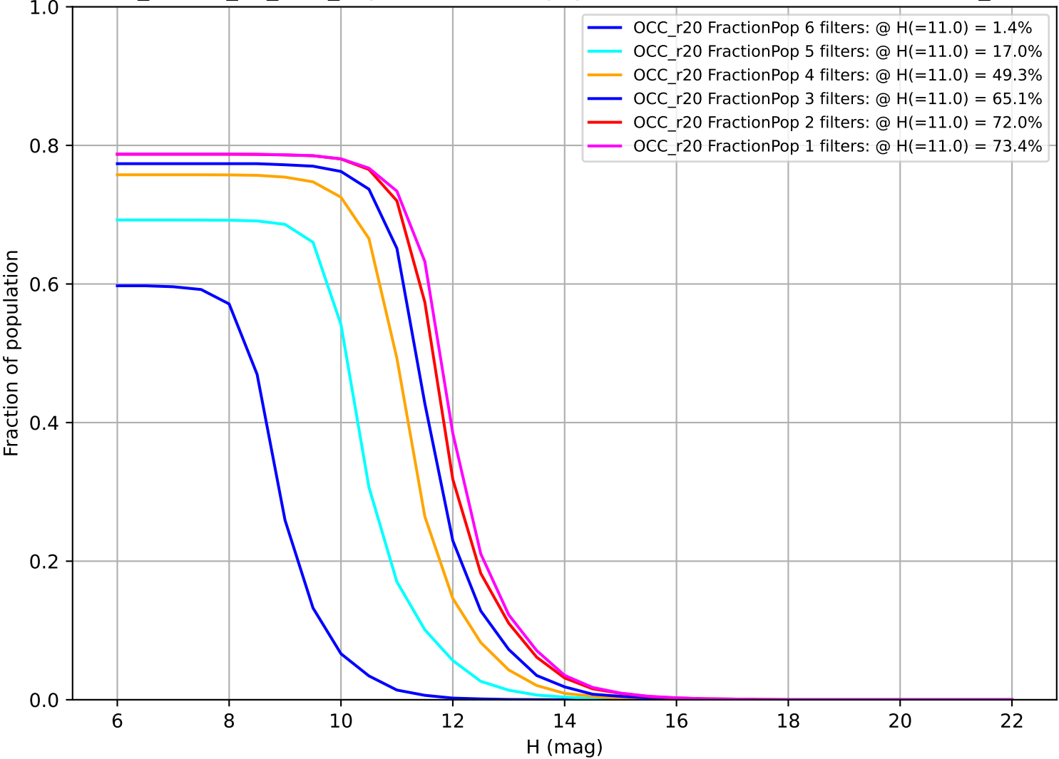
ddf_loaded_fl2_v3.4_10yrs: Fraction of population with colors in X filters OCC_r20
