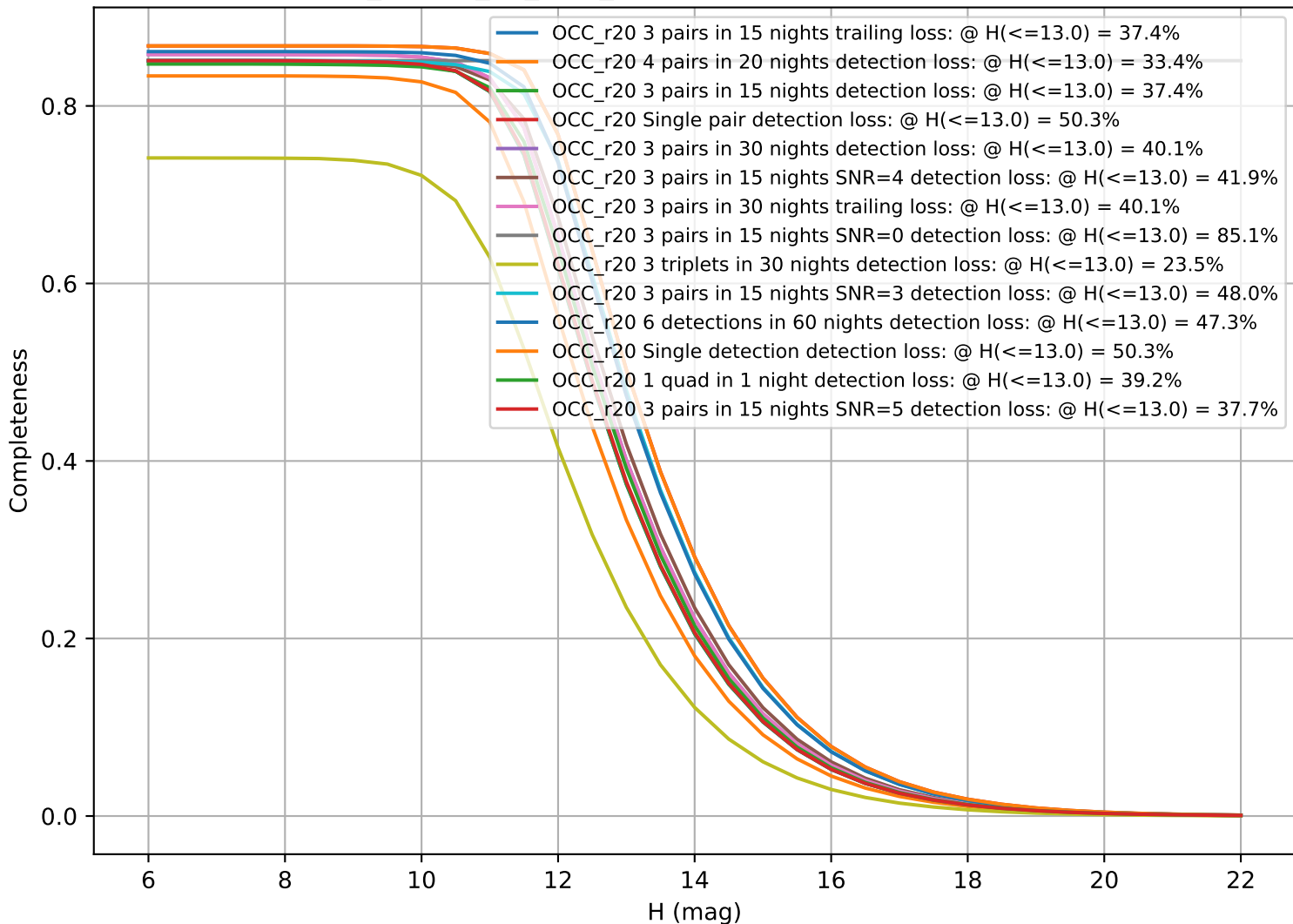
ddf_loaded_fl2_v3.4_10yrs: CumulativeCompleteness
