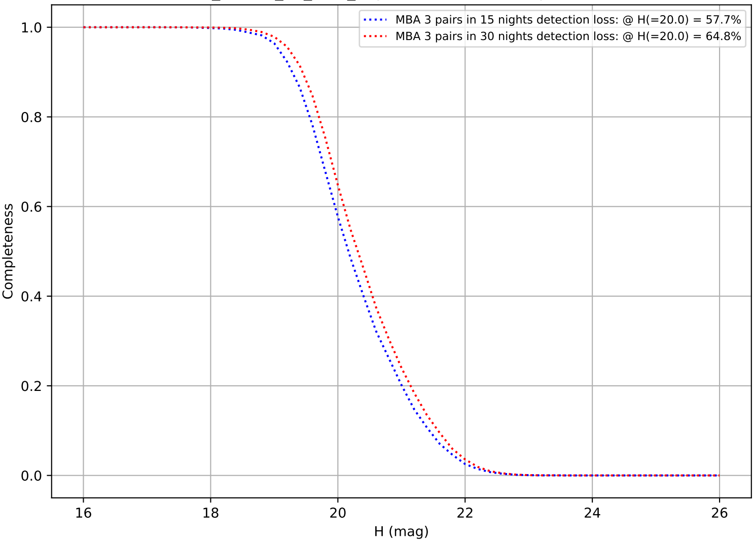
ddf_loaded_fl2_v3.4_10yrs: DifferentialCompleteness
