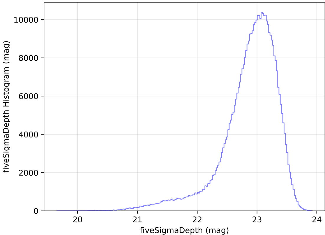
ddf_loaded_fl2_v3.4_10yrs z: fiveSigmaDepth Histogram
