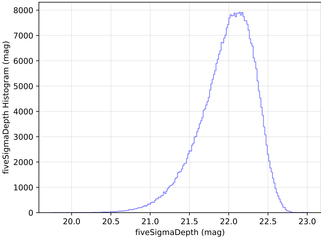
ddf_loaded_fl2_v3.4_10yrs y: fiveSigmaDepth Histogram
