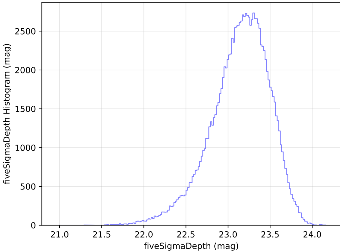
ddf_loaded_fl2_v3.4_10yrs u: fiveSigmaDepth Histogram
