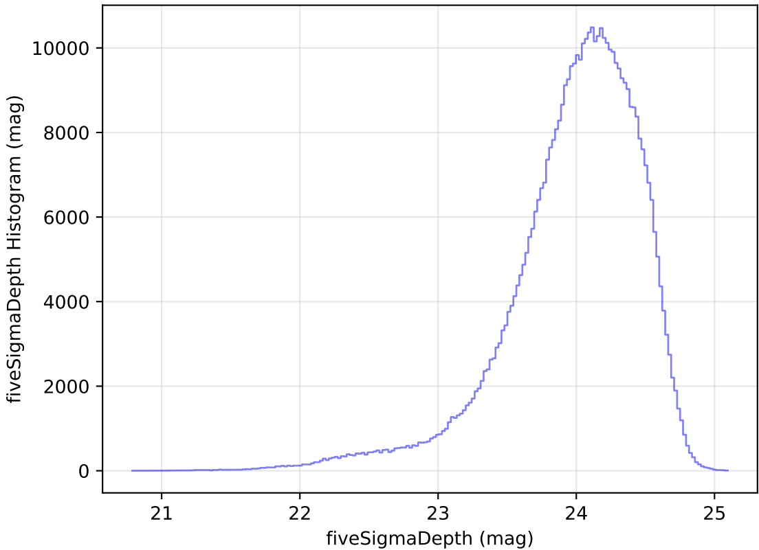
ddf_loaded_fl2_v3.4_10yrs r: fiveSigmaDepth Histogram
