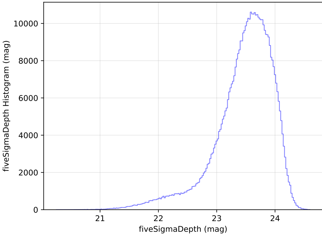
ddf_loaded_fl2_v3.4_10yrs i: fiveSigmaDepth Histogram
