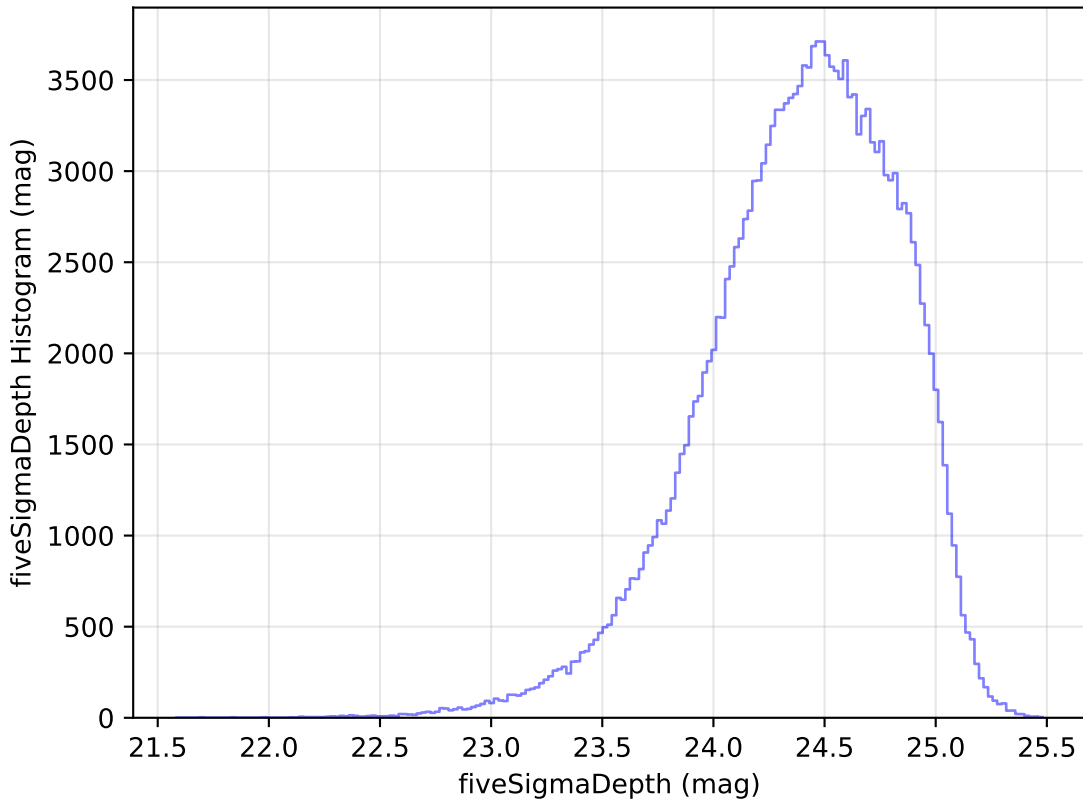
ddf_loaded_fl2_v3.4_10yrs g: fiveSigmaDepth Histogram
