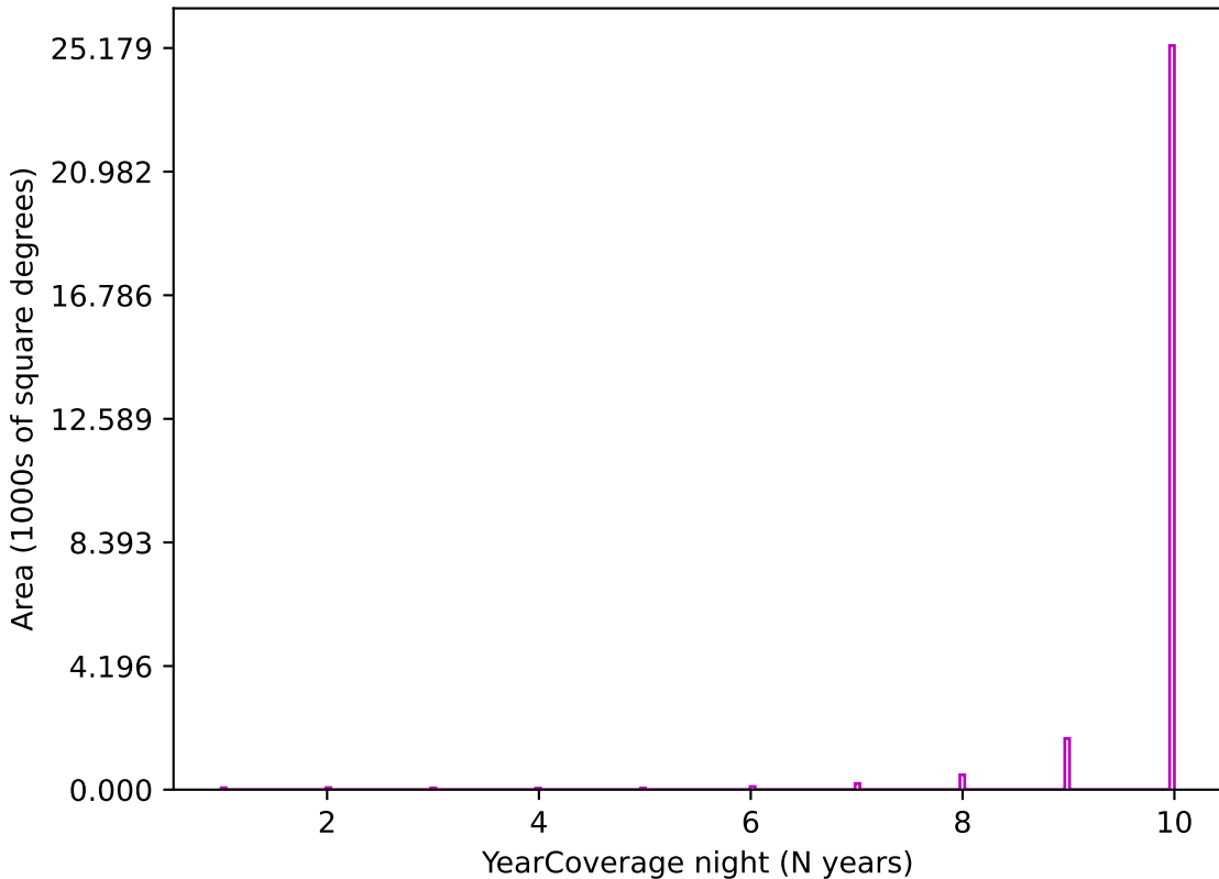
ddf_loaded_fl2_v3.4_10yrs z band: YearCoverage night
