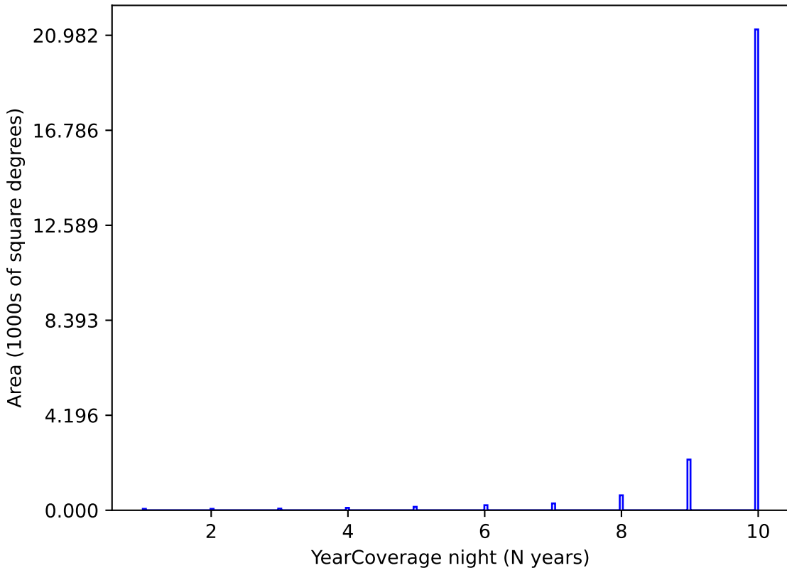
ddf_loaded_fl2_v3.4_10yrs y band: YearCoverage night
