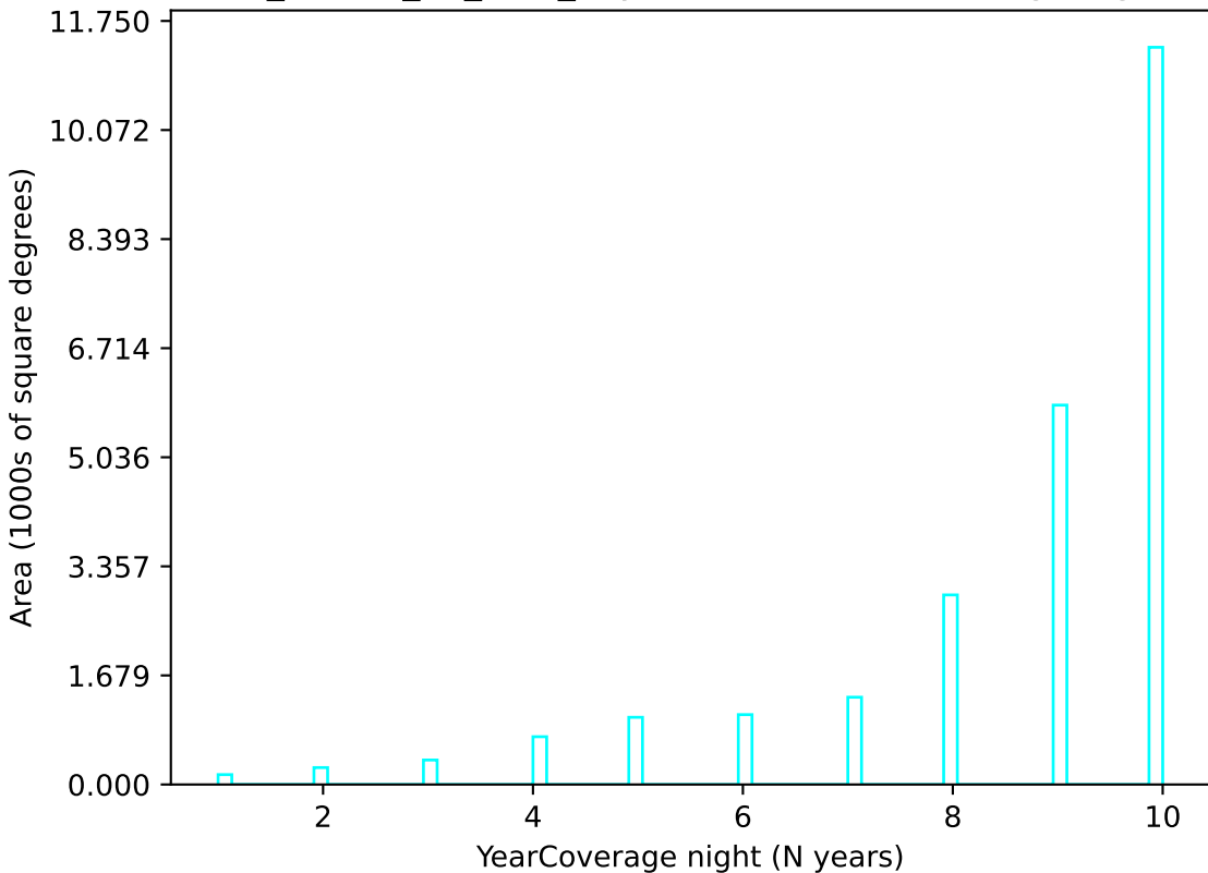
ddf_loaded_fl2_v3.4_10yrs u band: YearCoverage night
