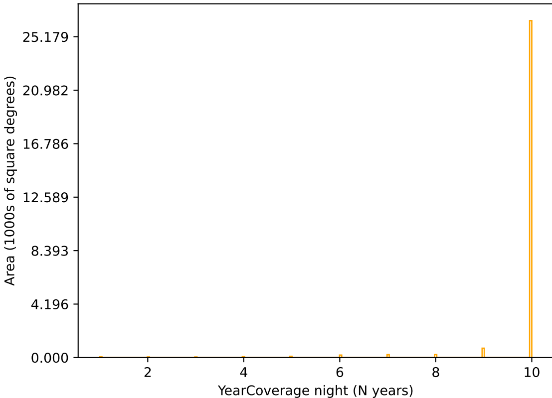
ddf_loaded_fl2_v3.4_10yrs r band: YearCoverage night
