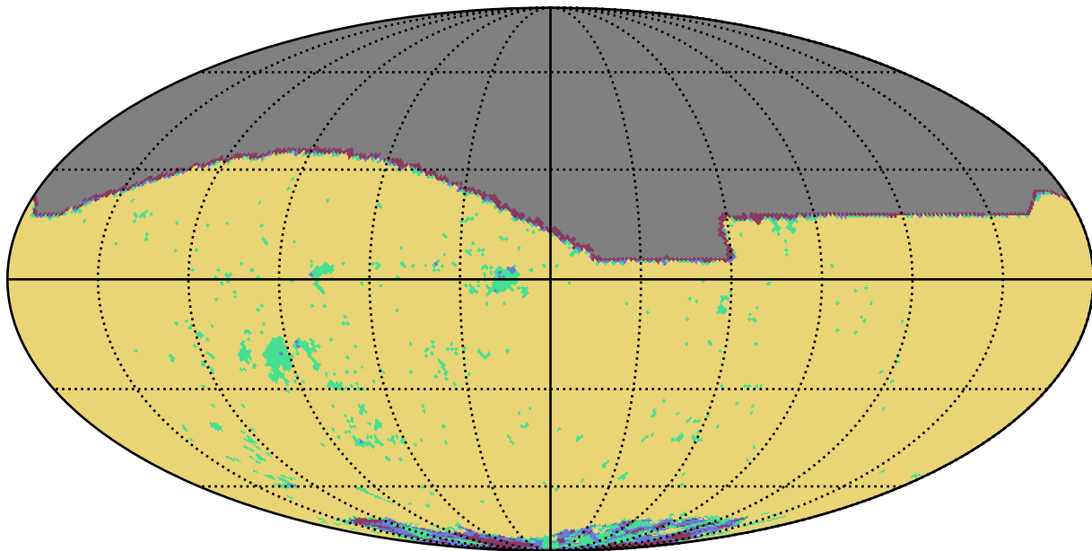
ddf_loaded_fl2_v3.4_10yrs i band: YearCoverage night
