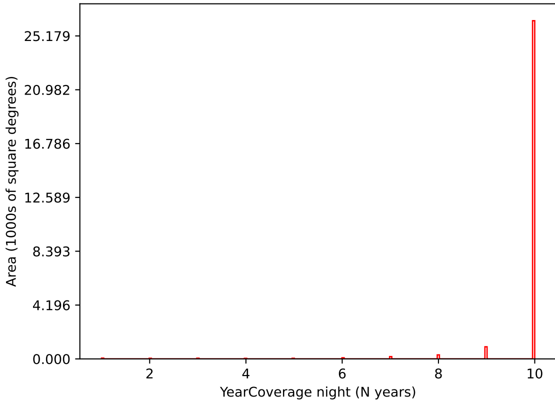
ddf_loaded_fl2_v3.4_10yrs i band: YearCoverage night
