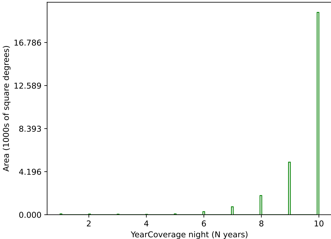
ddf_loaded_fl2_v3.4_10yrs g band: YearCoverage night
