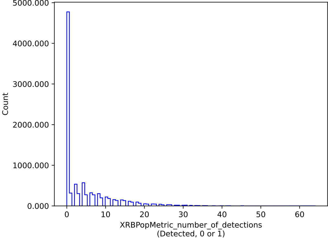
ddf_loaded_fl2_v3.4_10yrs : XRBPoMetric_number_of_detections
