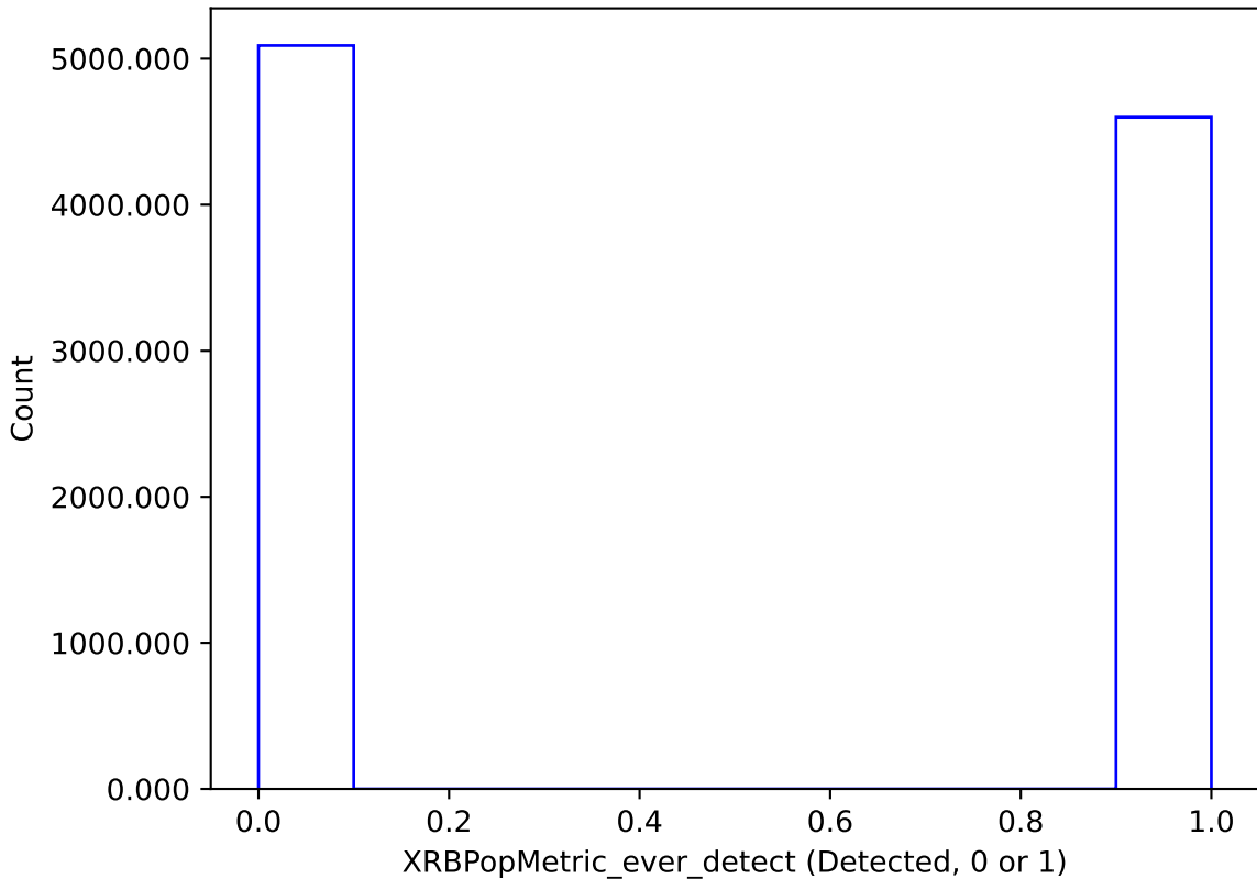
ddf_loaded_fl2_v3.4_10yrs : XRBPoMetric_ever_detect
