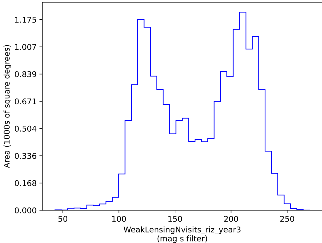
ddf_loaded_fl2_v3.4_10yrs gri band non-DD: WeakLensingNvisits_riz_year3
