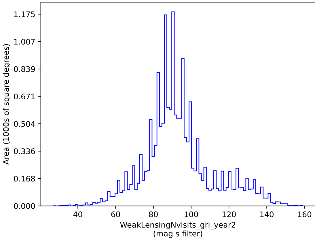
ddf_loaded_fl2_v3.4_10yrs gri band non-DD: WeakLensingNvisits_gri_year2
