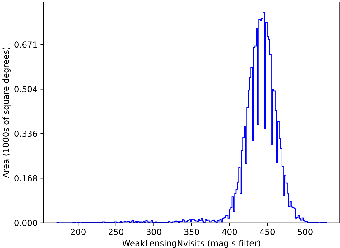
ddf_loaded_fl2_v3.4_10yrs gri band non-DD: WeakLensingNvisits
