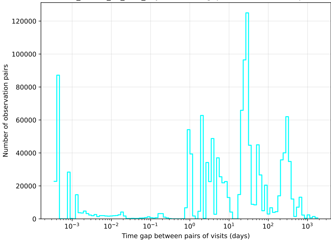
ddf_loaded_fl2_v3.4_10yrs u band: Tgaps observationStartMJD
