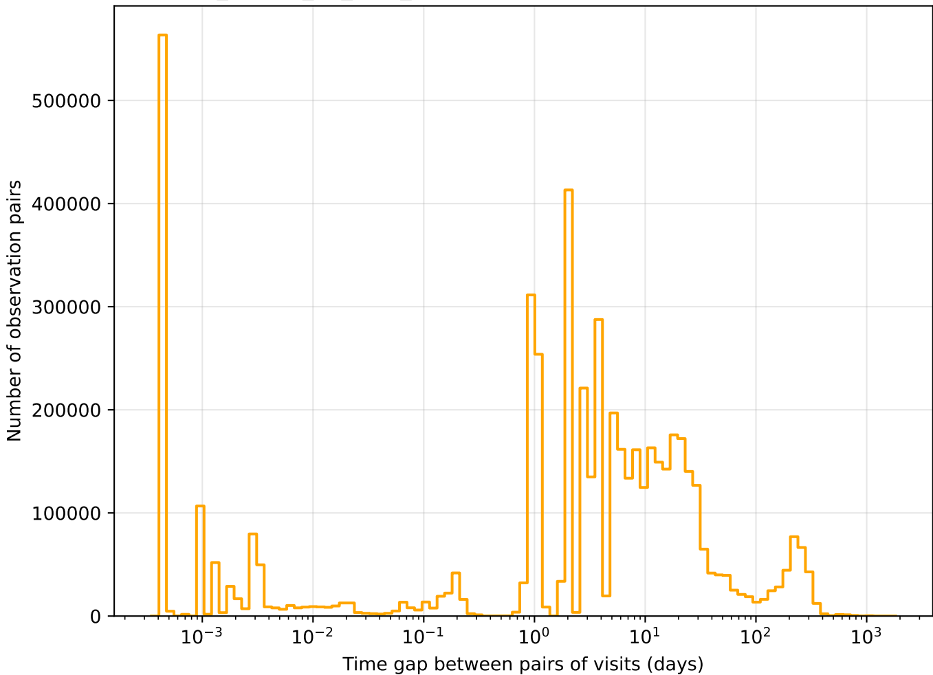
ddf_loaded_fl2_v3.4_10yrs r band: Tgaps observationStartMJD
