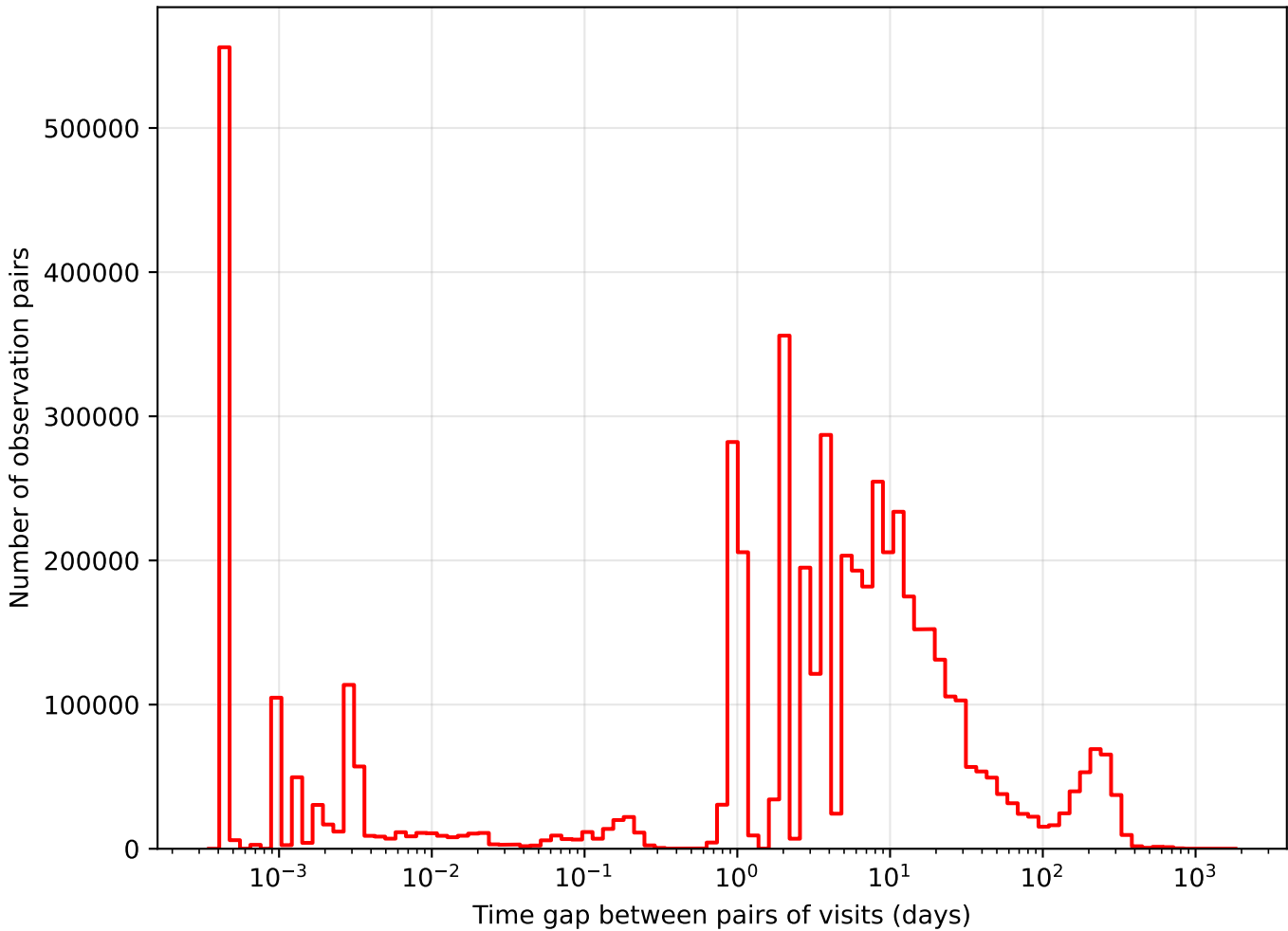
ddf_loaded_fl2_v3.4_10yrs i band: Tgaps observationStartMJD
