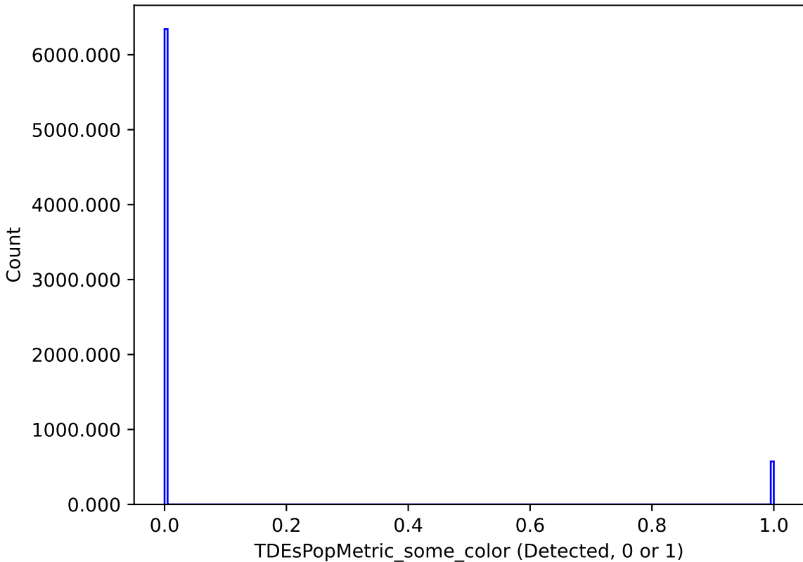
ddf_loaded_fl2_v3.4_10yrs : TDEsPopMetric_some_color
