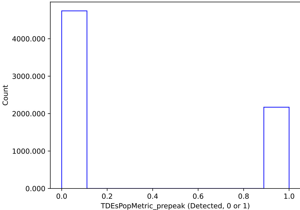
ddf_loaded_fl2_v3.4_10yrs : TDEsPopMetric_prepeak
