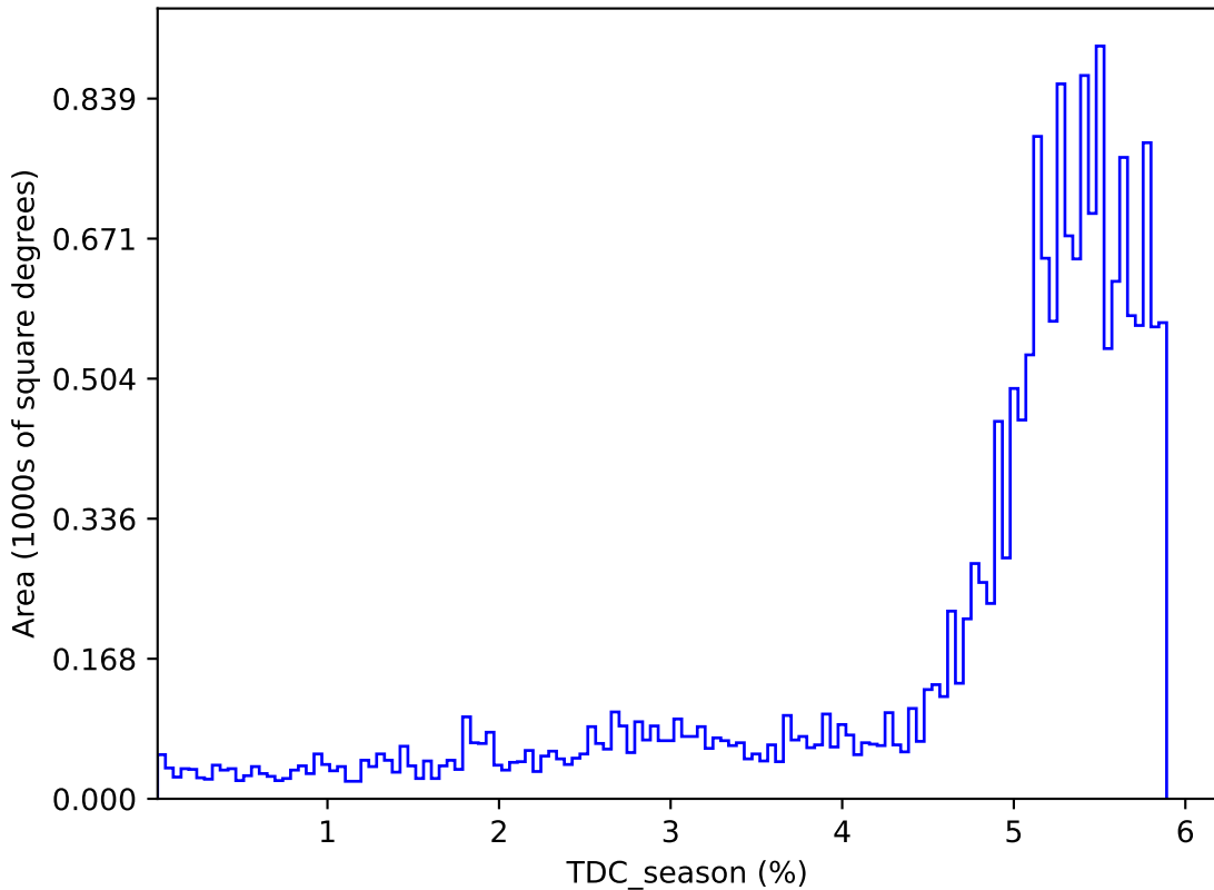
ddf_loaded_fl2_v3.4_10yrs : TDC_season
