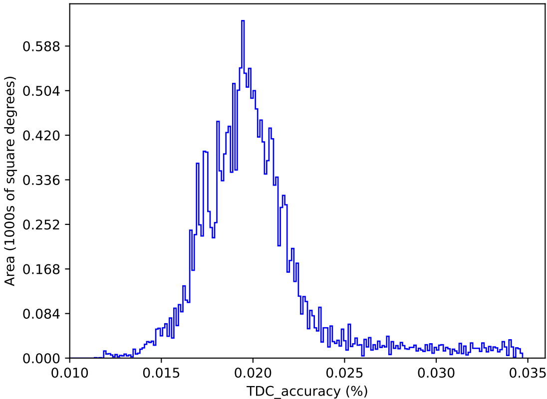
ddf_loaded_fl2_v3.4_10yrs : TDC_accuracy
