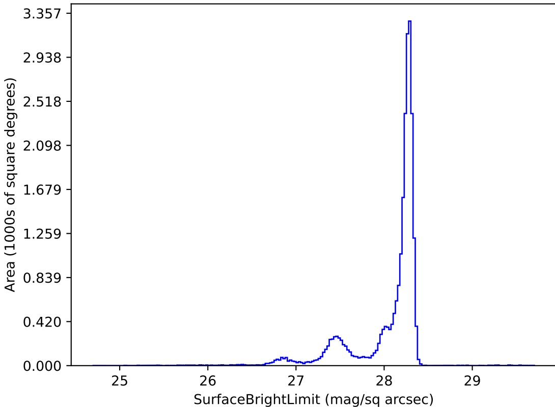
ddf_loaded_fl2_v3.4_10yrs y: SurfaceBrightLimit
