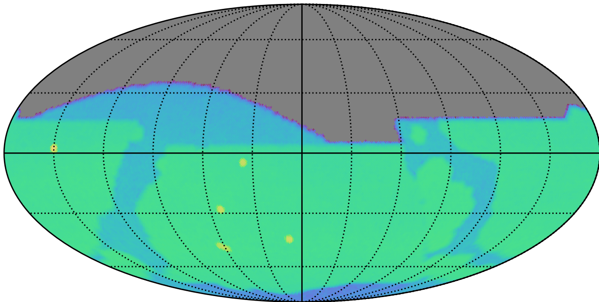
ddf_loaded_fl2_v3.4_10yrs r: SurfaceBrightLimit
