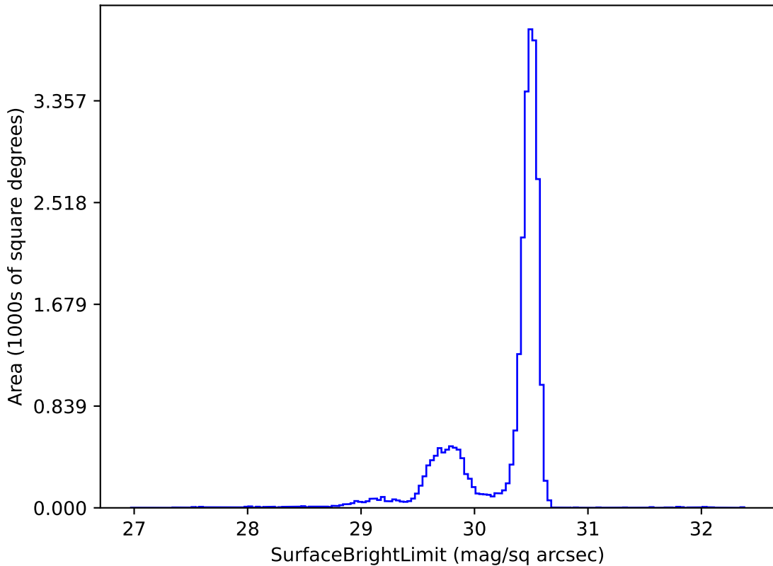
ddf_loaded_fl2_v3.4_10yrs r: SurfaceBrightLimit
