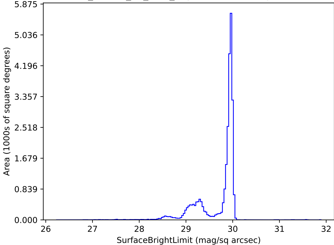
ddf_loaded_fl2_v3.4_10yrs i: SurfaceBrightLimit
