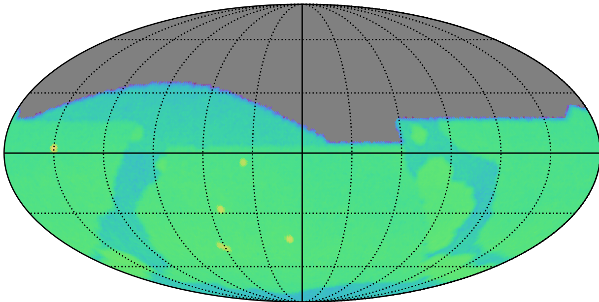
ddf_loaded_fl2_v3.4_10yrs g: SurfaceBrightLimit
