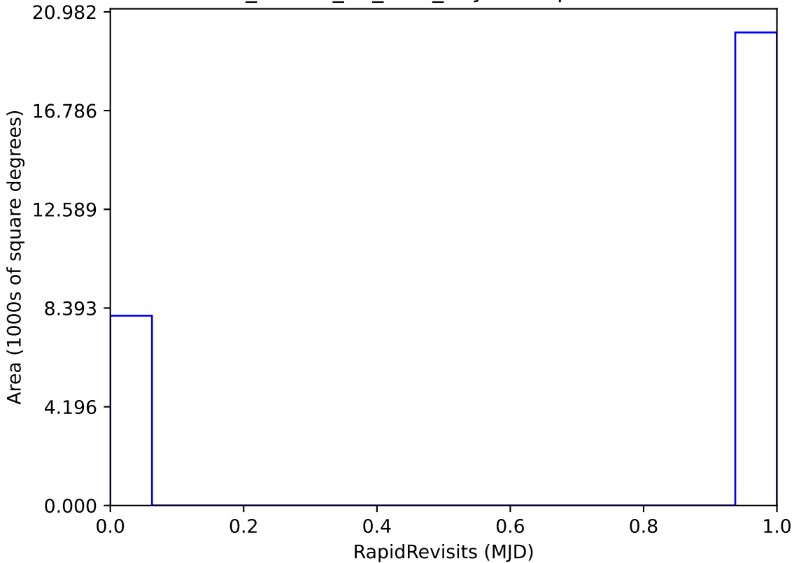
ddf_loaded_fl2_v3.4_10yrs : RapidRevisits
