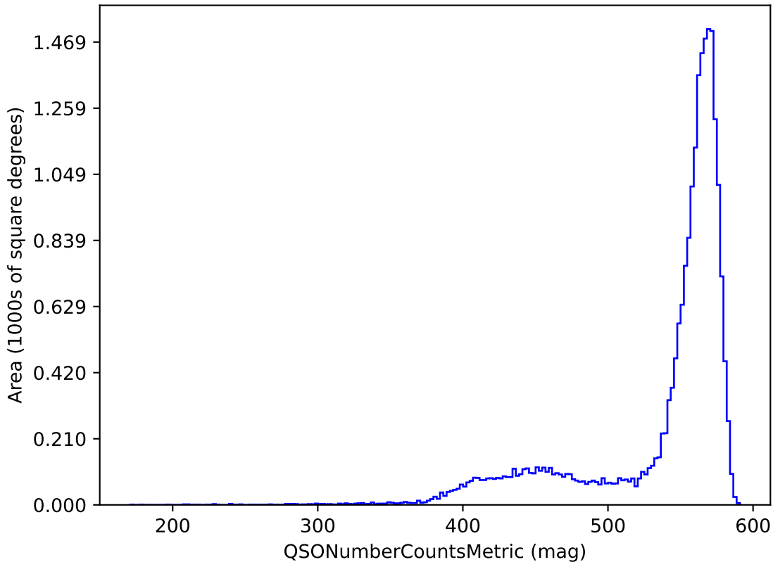
ddf_loaded_fl2_v3.4_10yrs y band and non-DD: QSONumberCountsMetric
