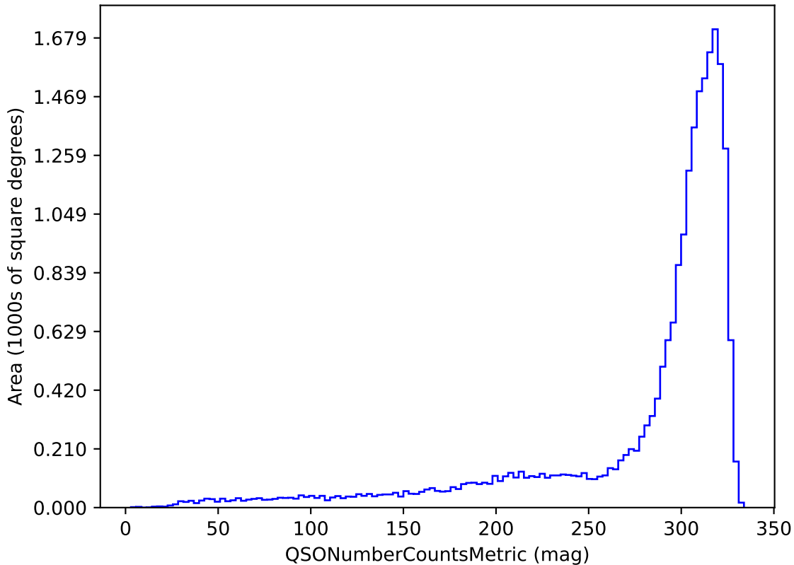
ddf_loaded_fl2_v3.4_10yrs u band and non-DD: QSONumberCountsMetric
