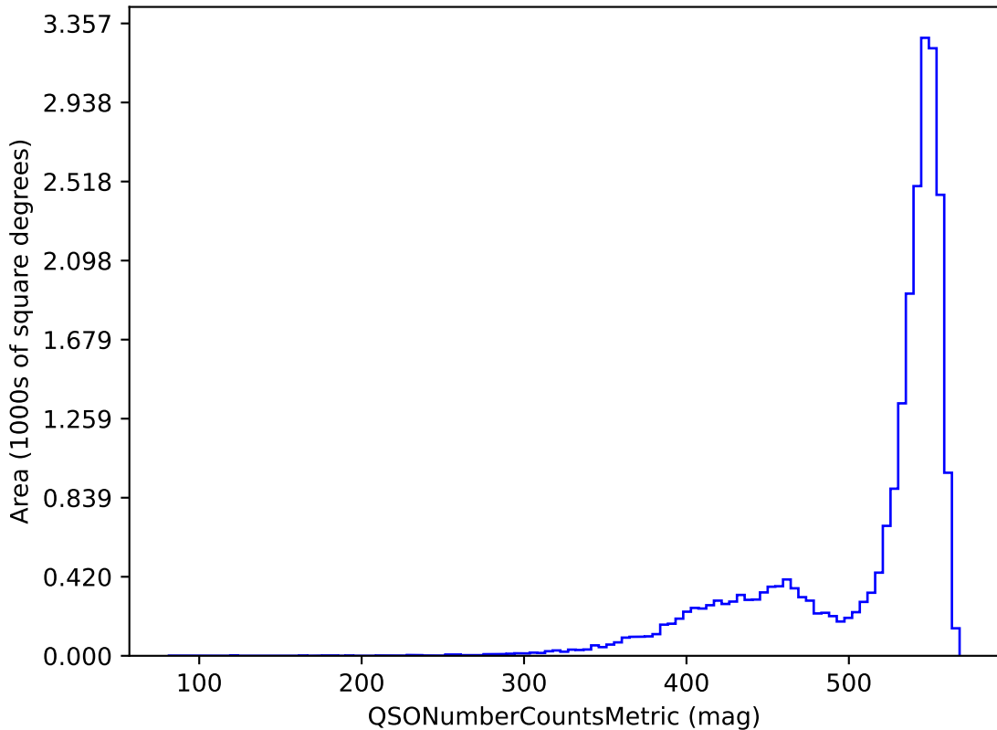
ddf_loaded_fl2_v3.4_10yrs i band and non-DD: QSONumberCountsMetric
